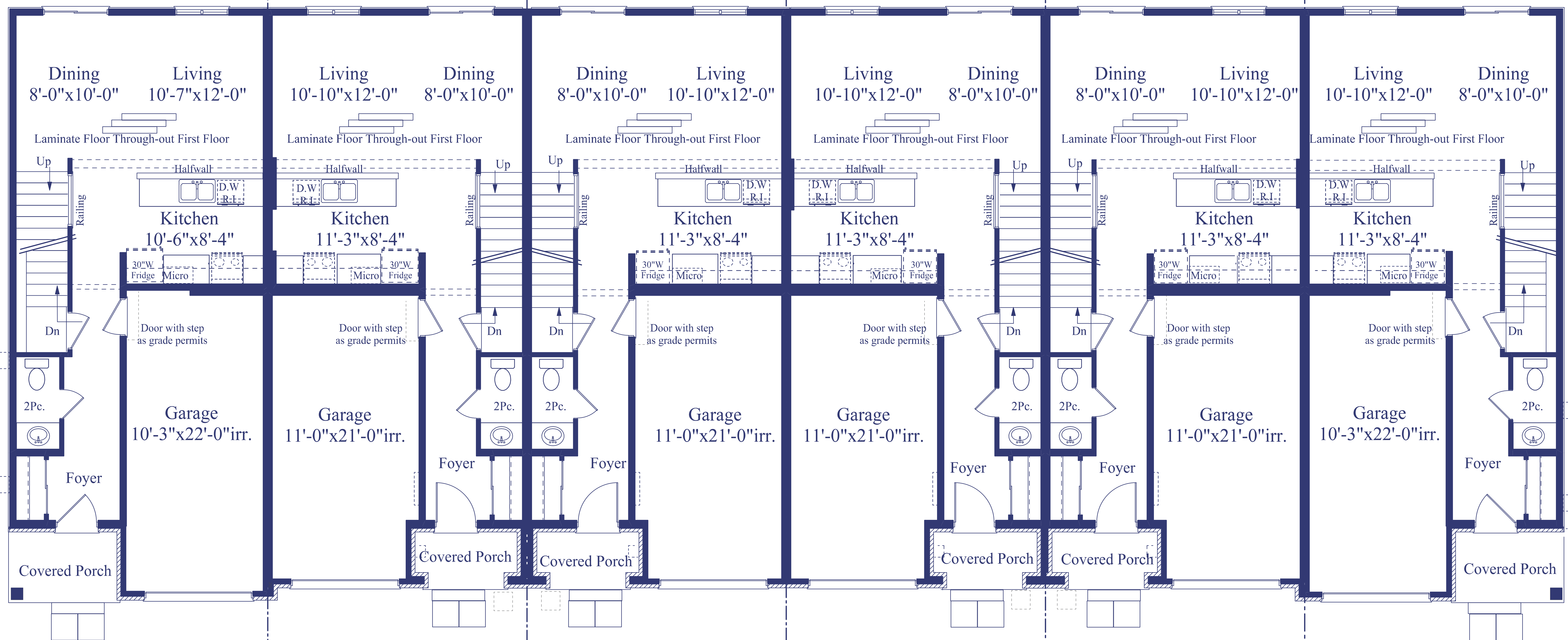
First floor plan
