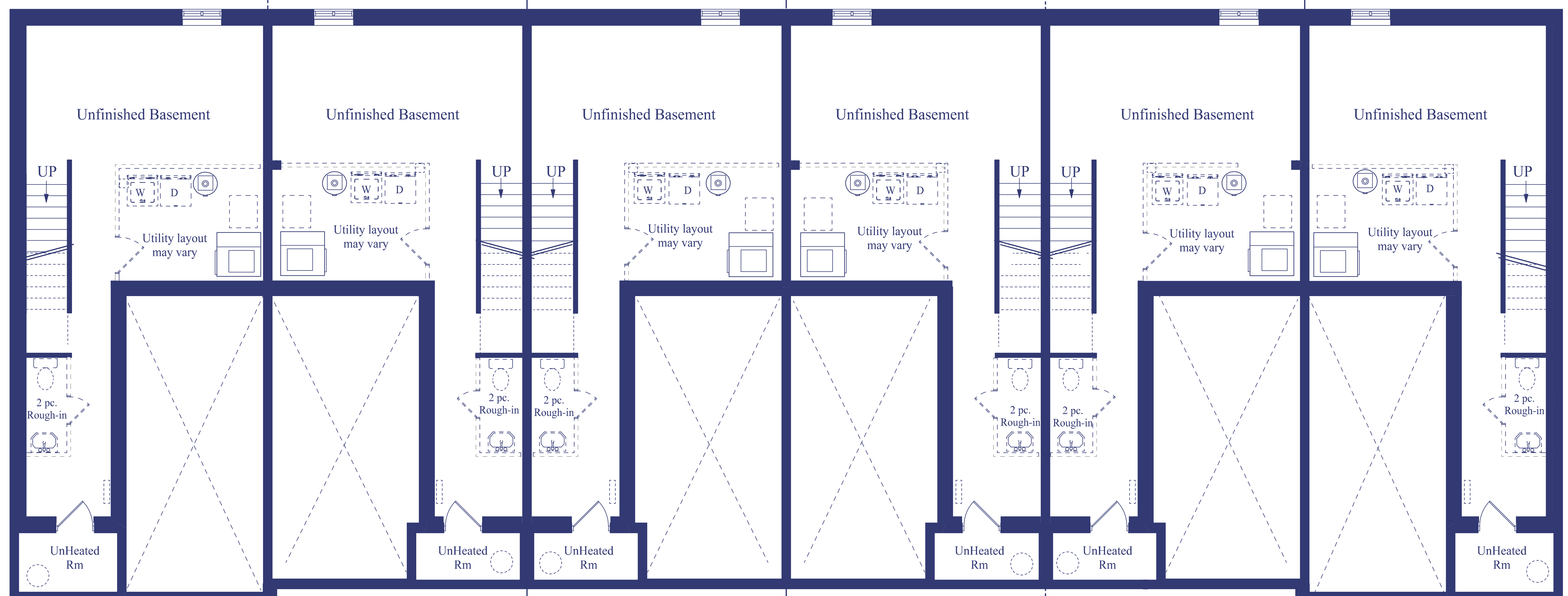
Basement floor plan
