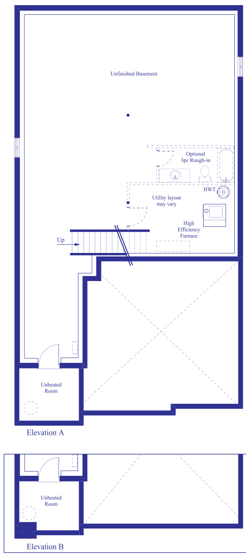
Basement
