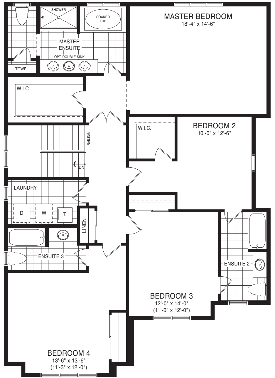
SECOND FLOOR PLAN STYLE A
