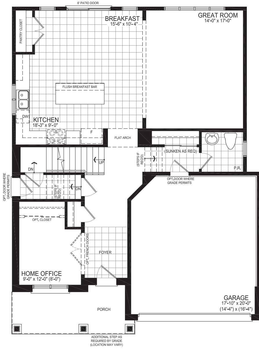
GROUND FLOOR PLAN STYLE A
