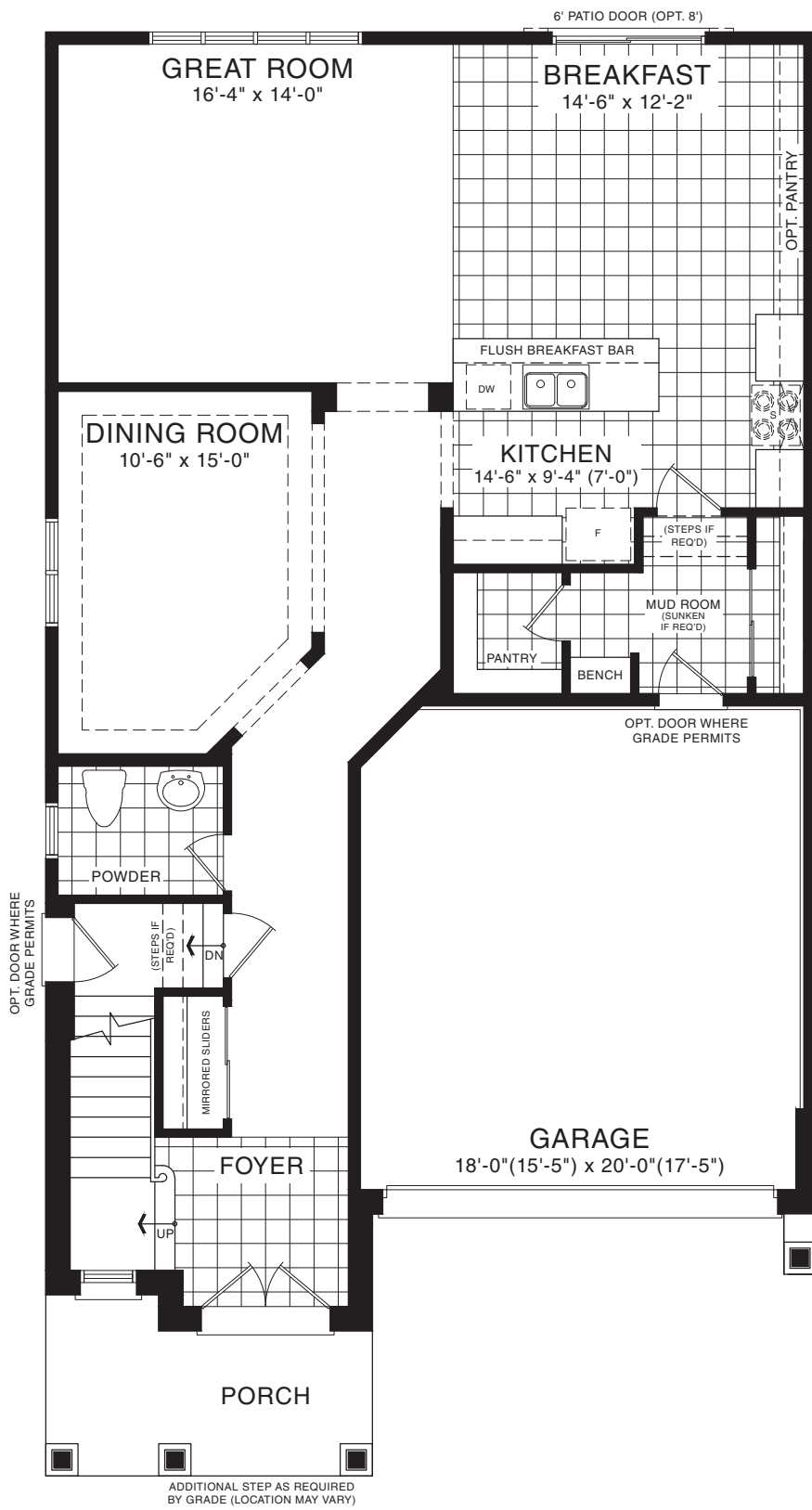
MAIN FLOOR PLAN STYLE A
