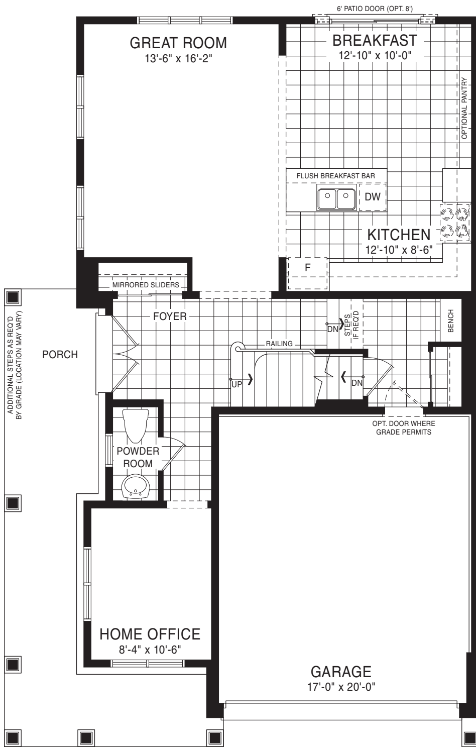
MAIN FLOOR PLAN STYLE A
