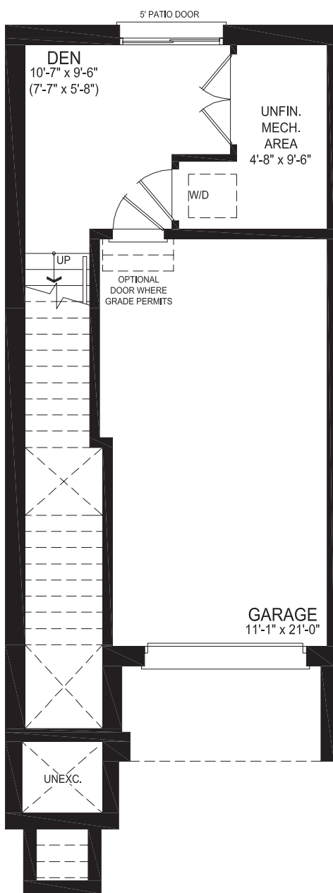
GROUND FLOOR PLAN STYLE A1 - END
