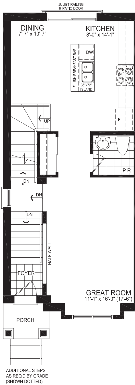
SECOND FLOOR PLAN STYLE A1 - END
