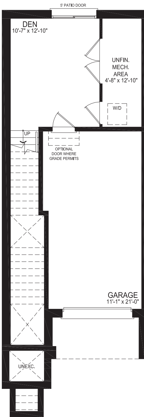
GROUND FLOOR PLAN STYLE A1
