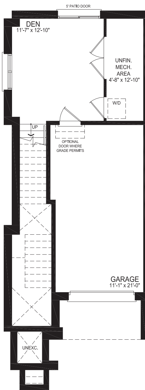
GROUND FLOOR PLAN STYLE A1
